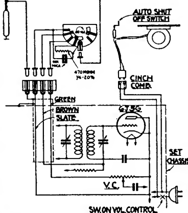
CIRCUIT #78 MODEL 95-307 CHASSIS #5907
