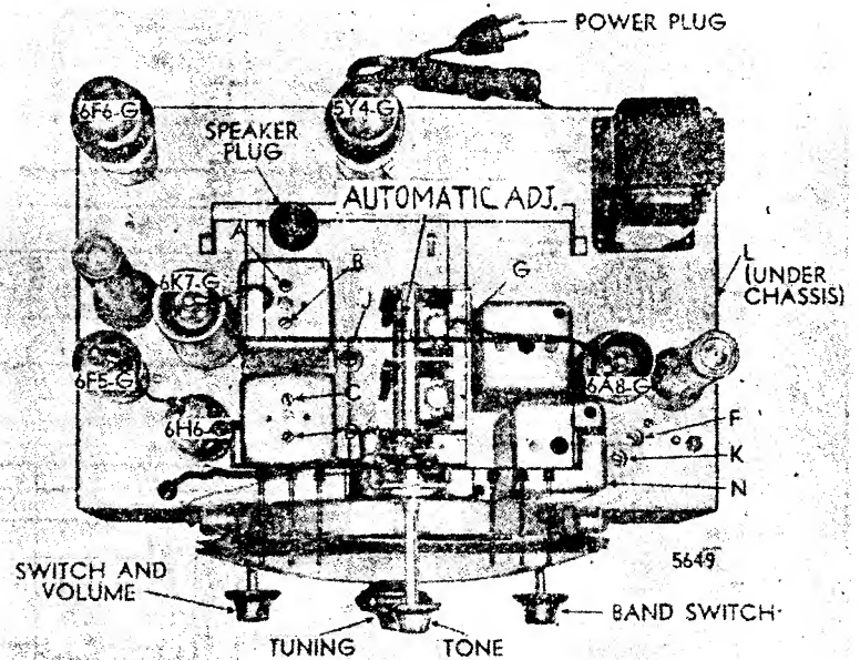
Location of Tubes and Trimmers
