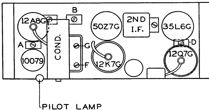
Location of Tubes and Trimmers
