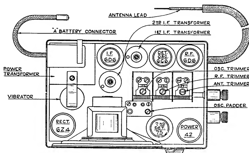
Fig. 1—TUBE POSITION
