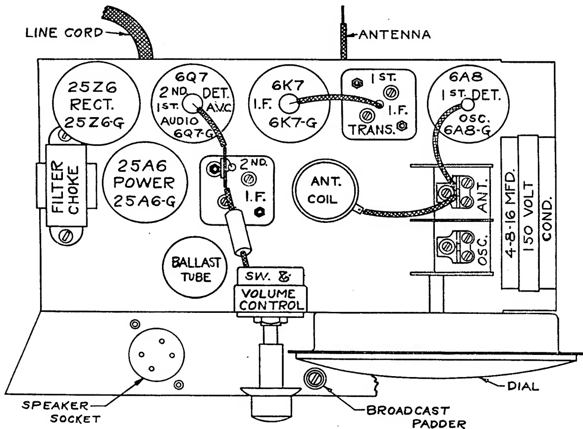
LOCATION OF TRIMMERS
