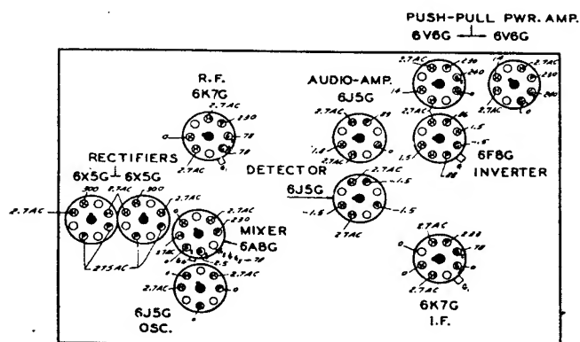
Location of Tubes and Trimmers
