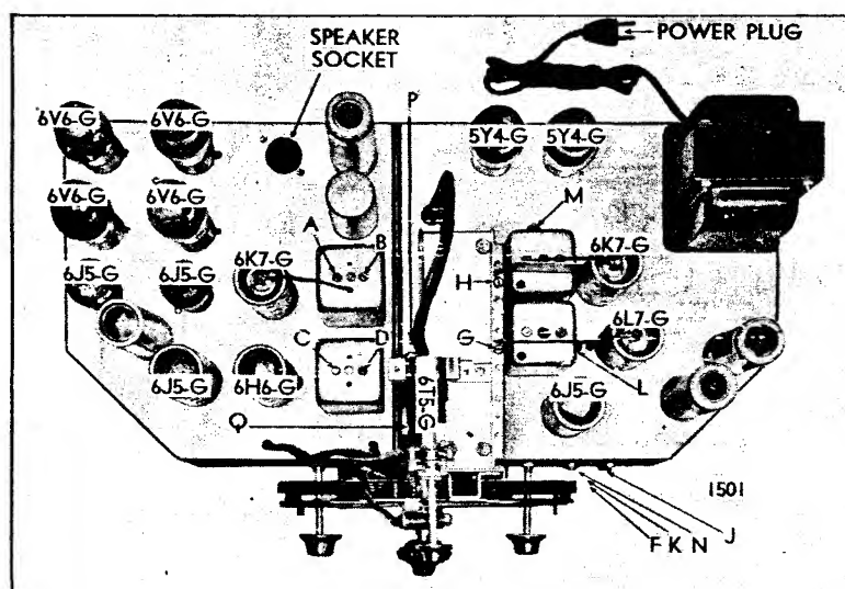
LOCATION OF TRIMMERS
