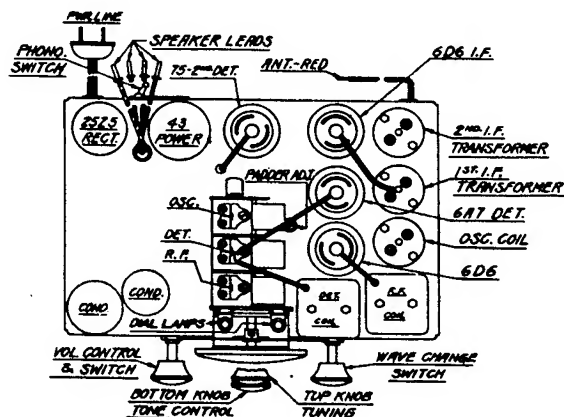
Tube Position
