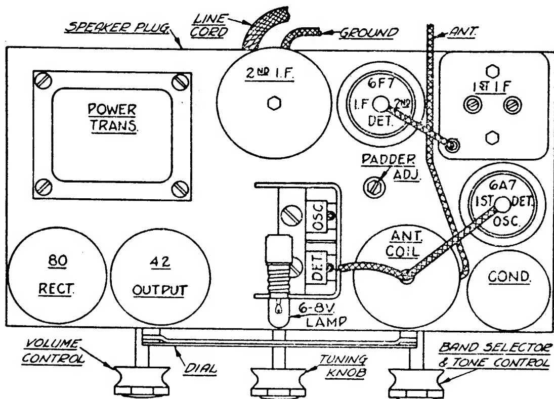
Tube Position
