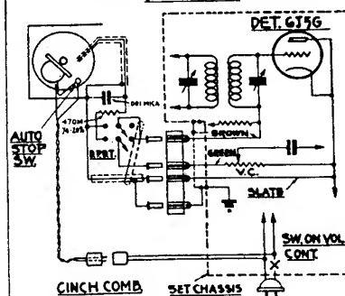
MODEL #65-301 & MODEL #65-305 CHASSIS #9651
