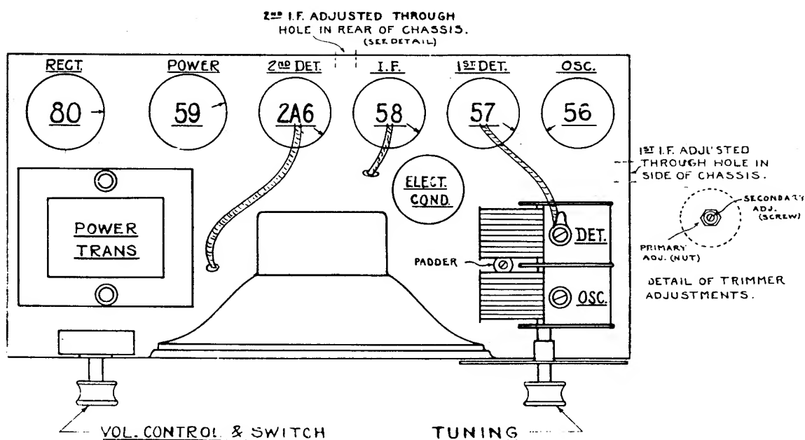
Tube Position
