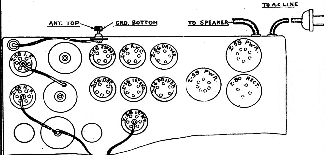
TUBE LAYOUT
