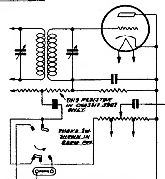
CIRCUIT #2A
