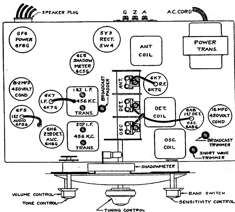
TUBE POSITION
