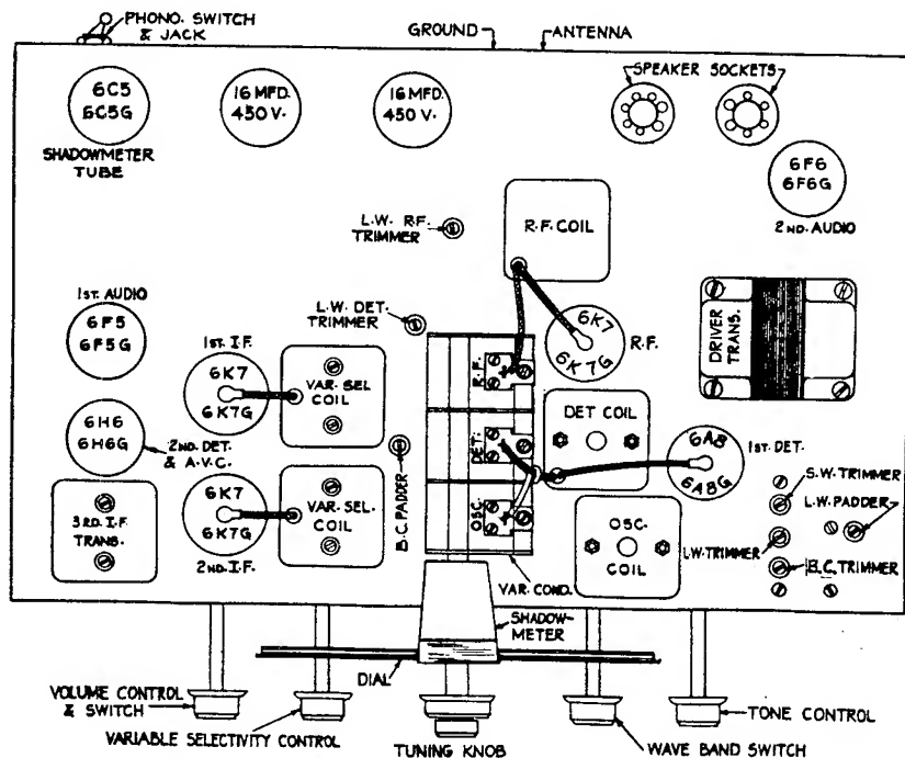
Receiver Chassis Drawing
