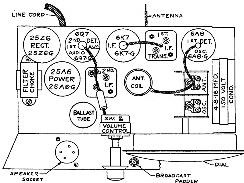
TUBE POSITION
