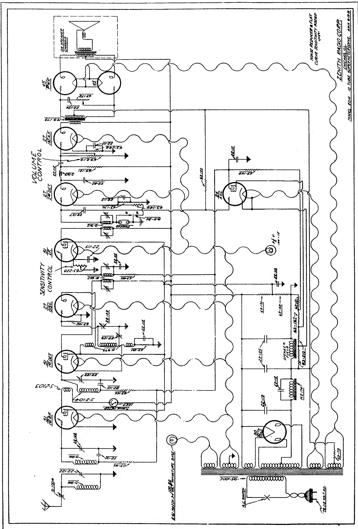
Fig. 1—CIRCUIT DIAGRAM—MODELS 91 After No. 375,532, 92 After No. 302,007
