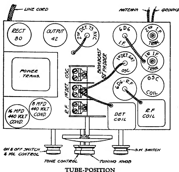
Tube Position
