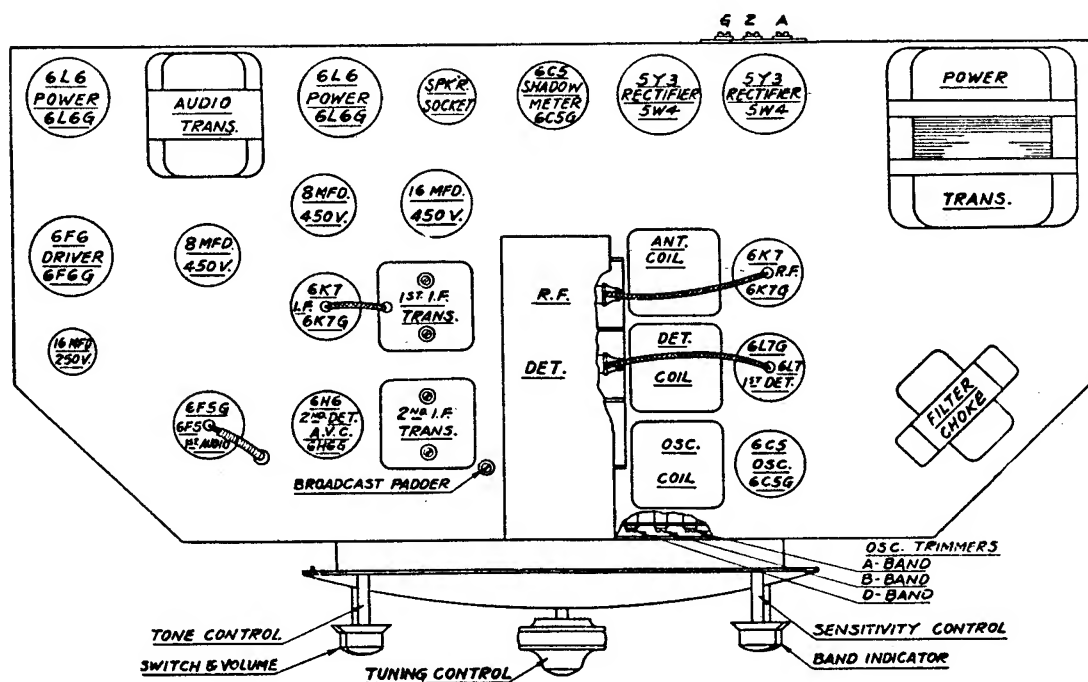
LOCATION OF TRIMMERS
