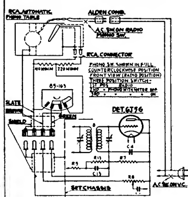
CIRCUIT #78 MODEL 95-307 CHASSIS #5907
