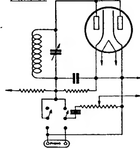
CIRCUIT 24
