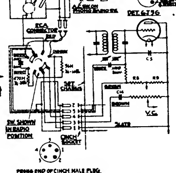
CIRCUIT #2A
