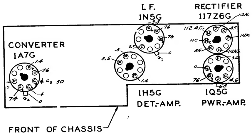
Socket Voltages
