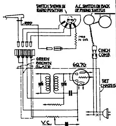
CIRCUIT #5A MODEL-65-306 CHASSIS #5651
