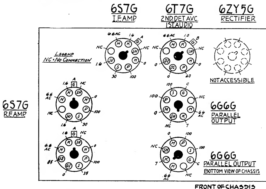
SOCKET VOLTAGES
