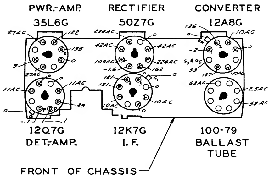
Socket Voltages
